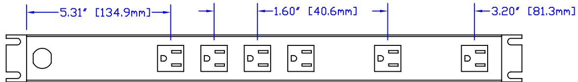
BOTTOM VIEW
